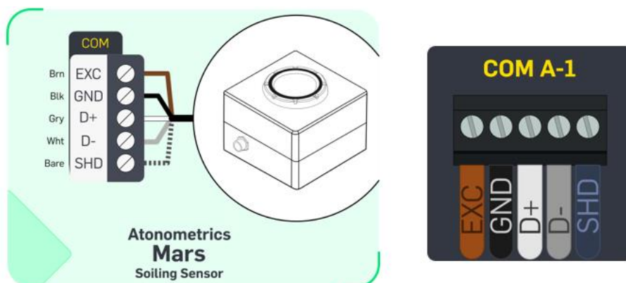
Figure 11: Mars™ Wiring Diagrams
